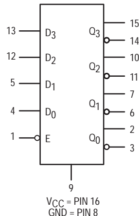
LOGIC SYMBOL
