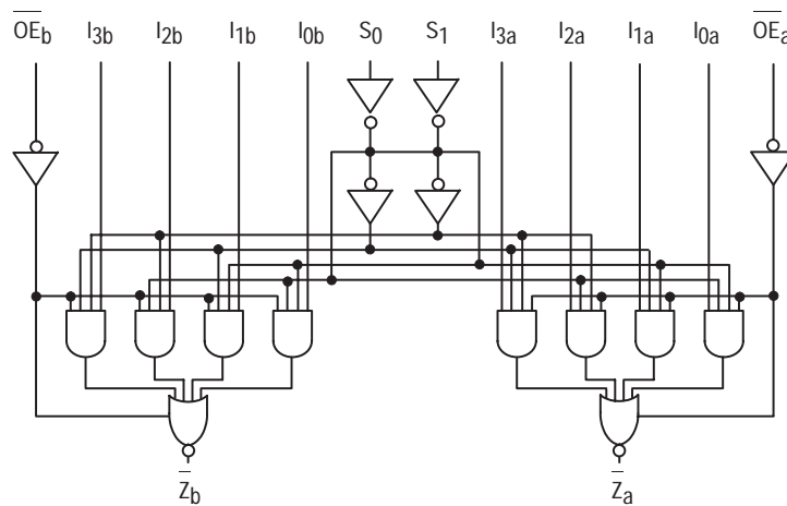
LOGIC DIAGRAM
