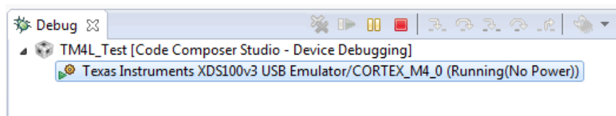
Figure 44. CPU Core Status Display Indicating Deep Sleep Mode
