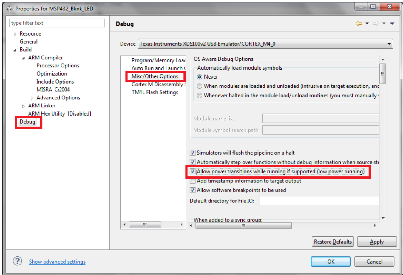
Figure 43. Enabling Low Power Run
