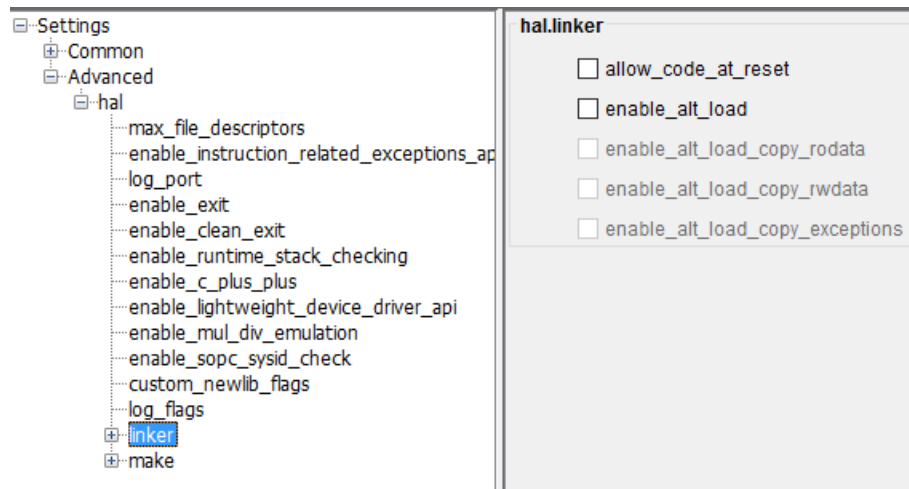
Figure 198. Advanced.hal.linker Settings
