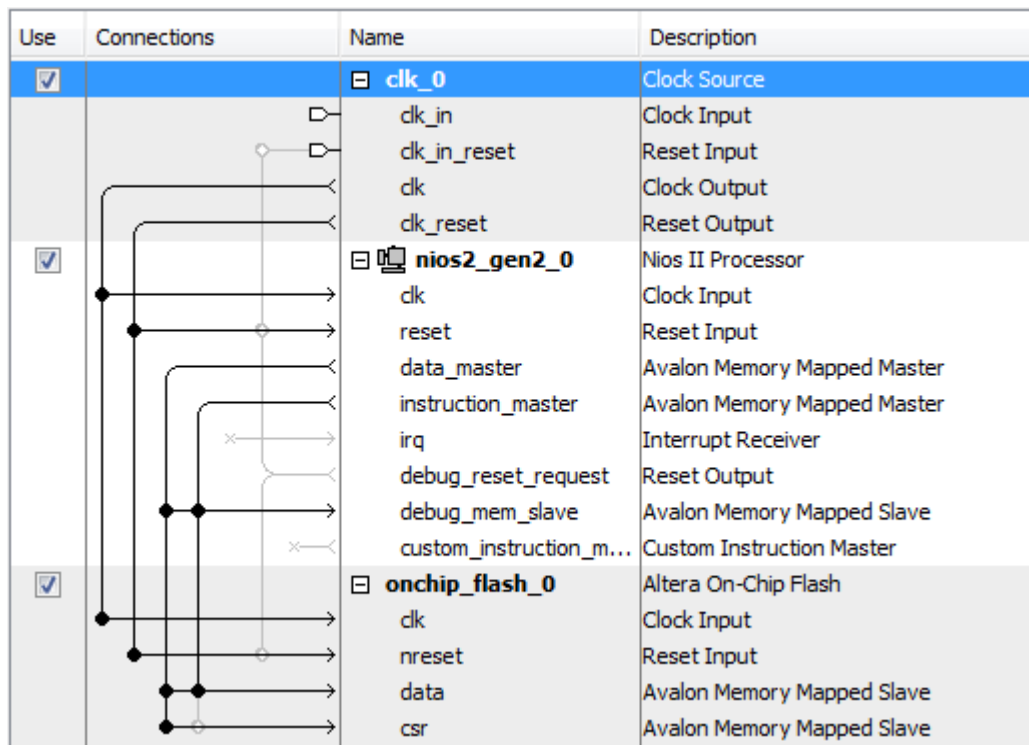
Figure 50. Connection Example for The On-chip Flash IP and the Nios II Processor
