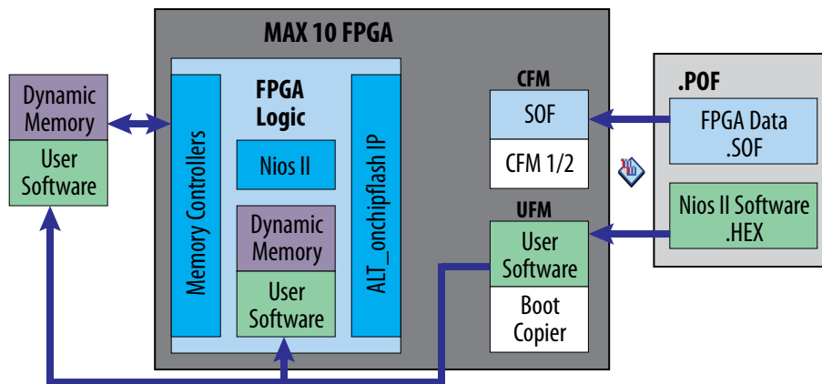
Figure 70. Block Diagram
