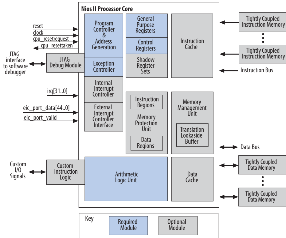
Figure 2. Nios II Processor Core Block Diagram
