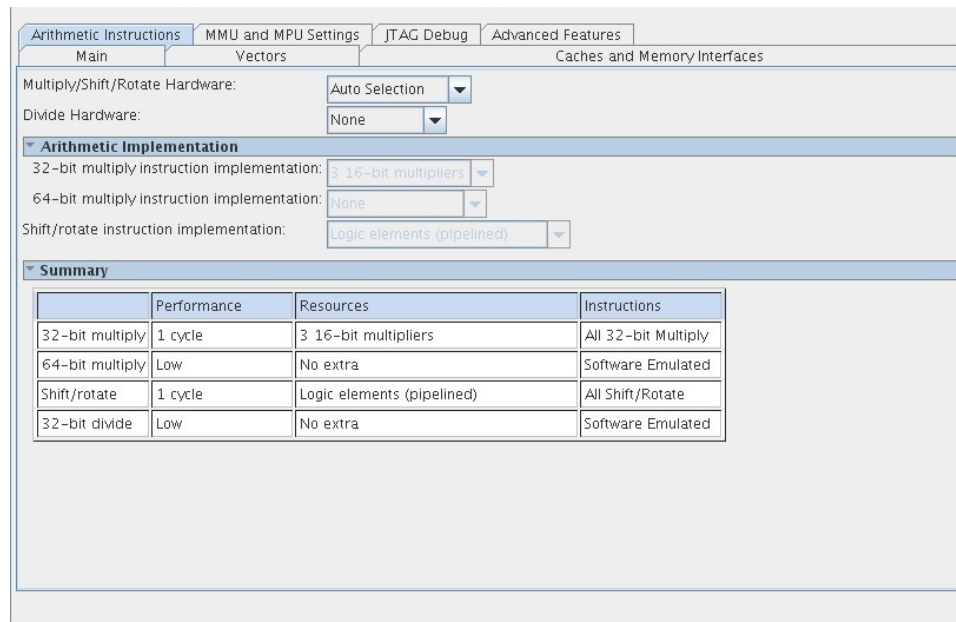
Figure 9. Nios II Platform Designer Arithmetic Instructions Tab
