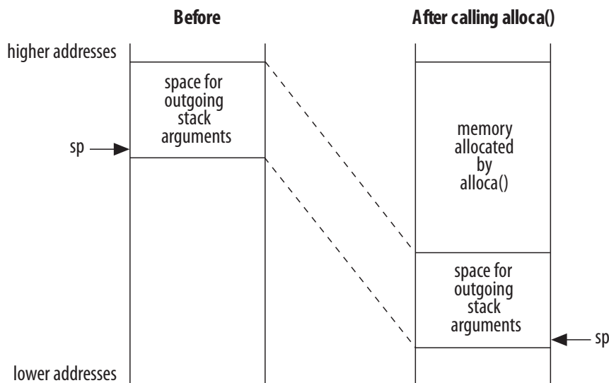
Figure 14. Stack Frame after Calling alloca()
