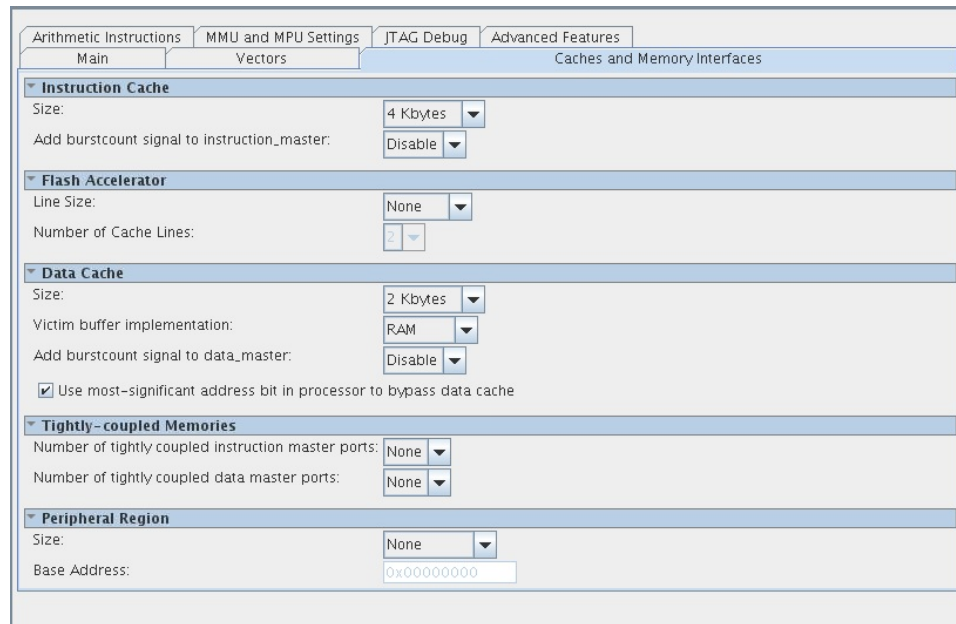
Figure 8. Nios II Platform Designer Caches and Memory Interfaces Tab
