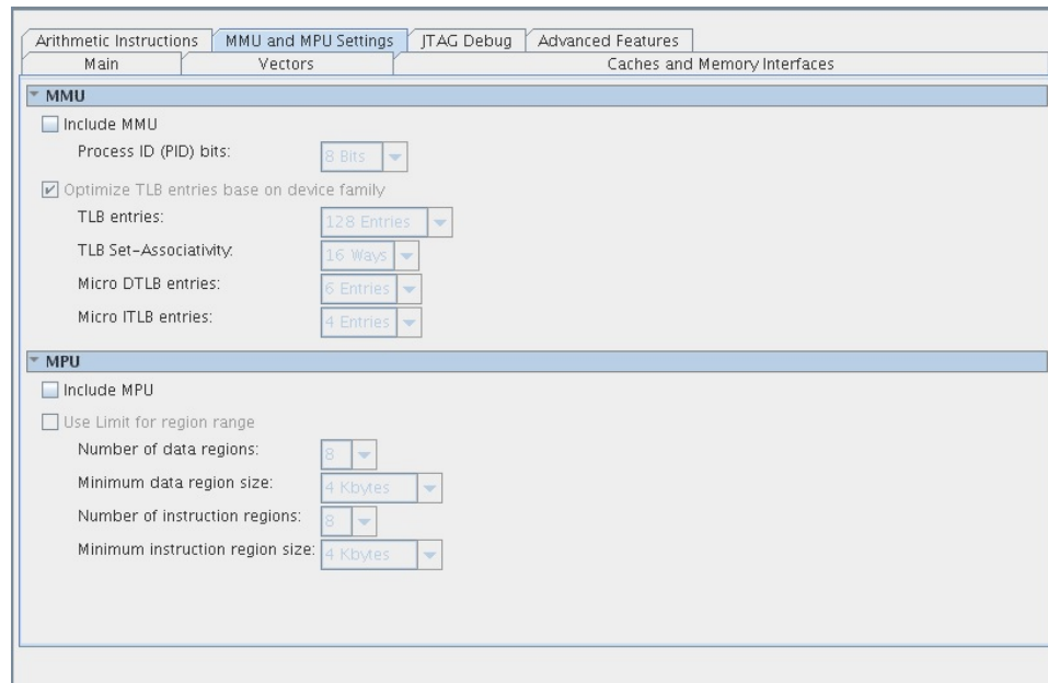
Figure 10. Nios II Platform Designer MMU and MPU Settings Tab
