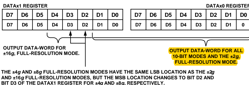
Figure 48. Data Formatting of Full-Resolution and \pm 2 g, 10-Bit Modes of Operation When Output Data Is Right Justified
