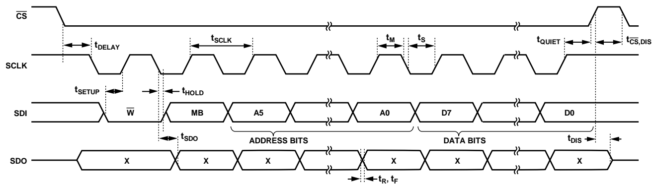
Figure 36. SPI 4-Wire Write
