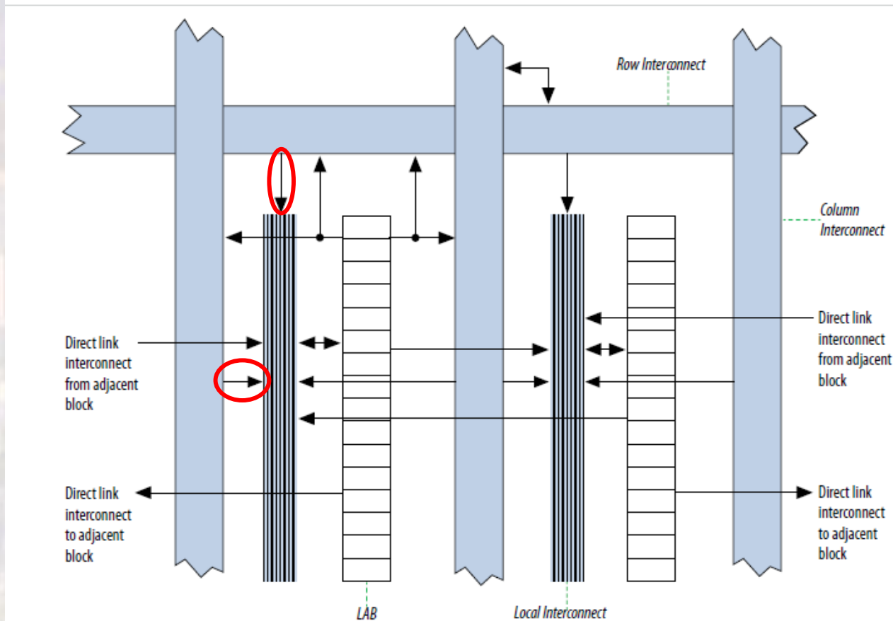
Figure 2: LAB Structure of MAX 10 Devices
