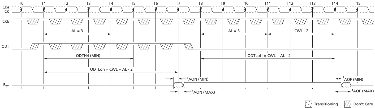
Figure 115: Synchronous ODT
