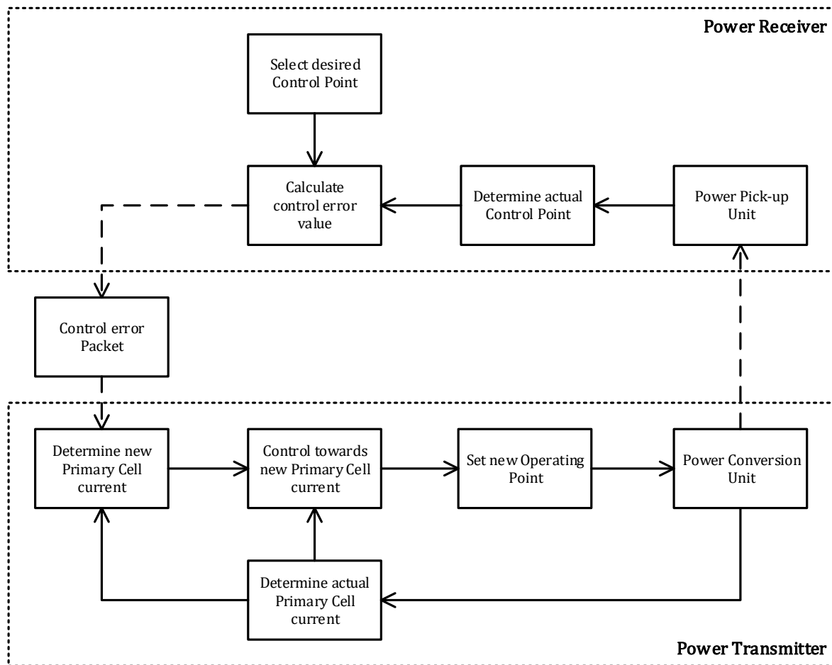
Figure 17. Power transfer control loop
