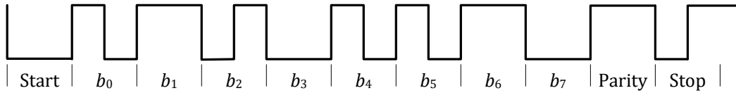
Figure 41. Example of the asynchronous serial format
