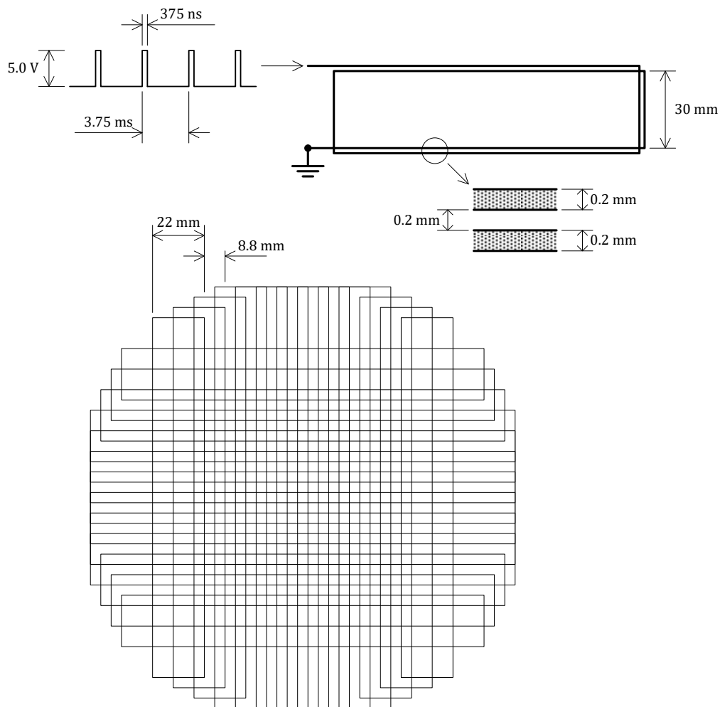
Figure 53. Detection Coil
