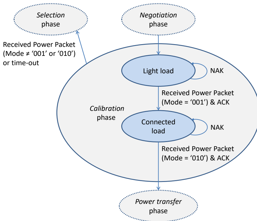
Figure 23. State diagram of the calibration phase
