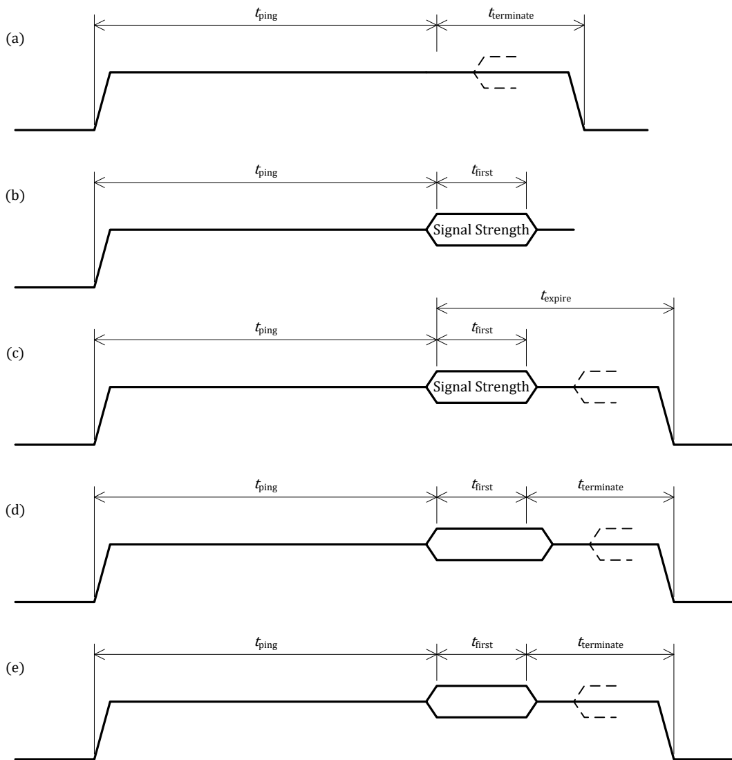
Figure 19. Power Transmitter timing in the ping phase
