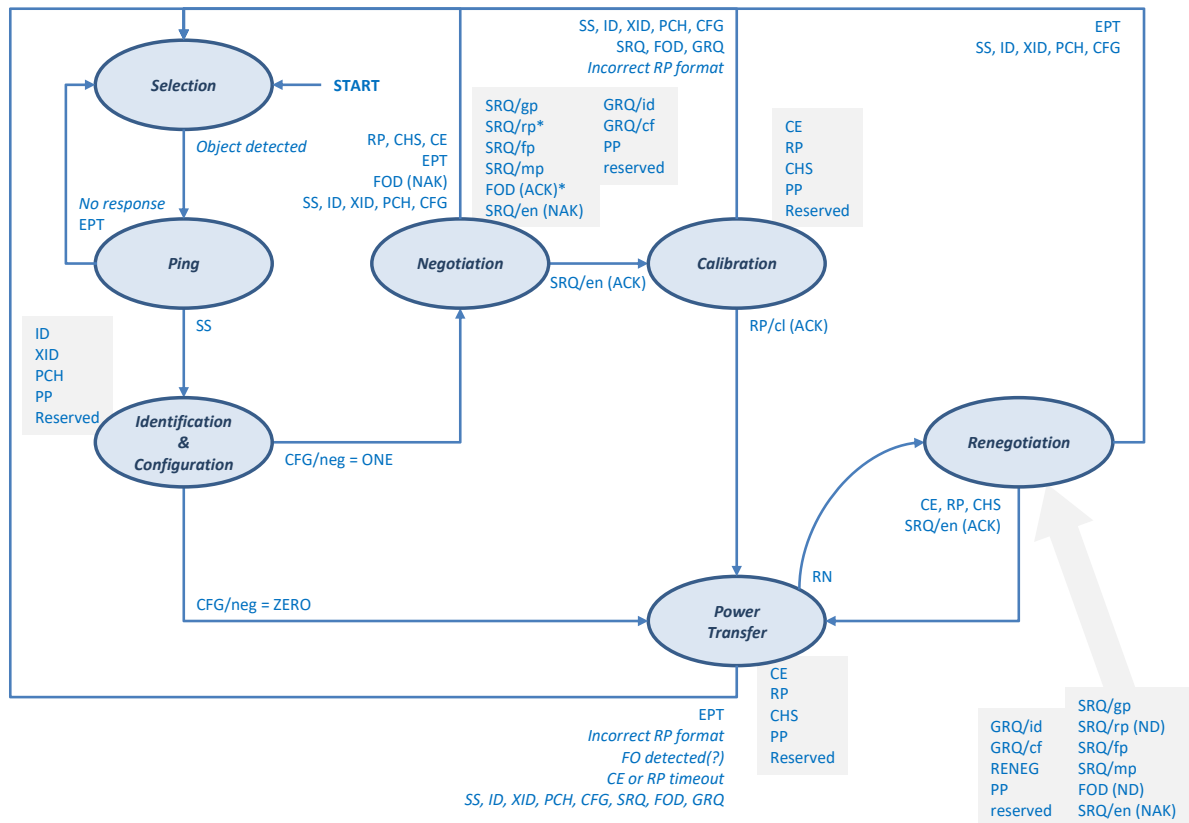
Figure 34. State diagram
