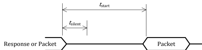
Figure 31. Power Receiver timing in the negotiation phase (transmit)
