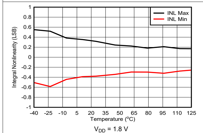
Figure 7-4. Integral Nonlinearity vs Temperature
