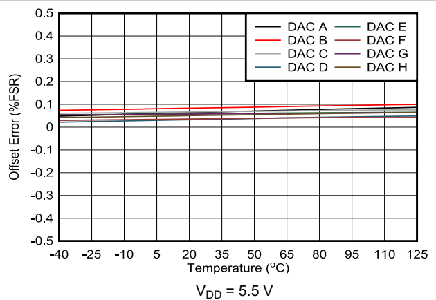
Figure 7-25. Offset Error vs Temperature
