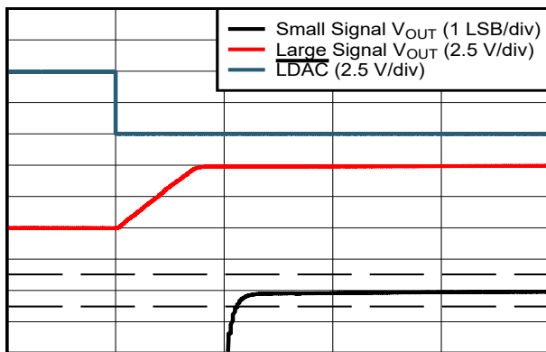
Figure 7-36. Glitch Impulse, Rising Edge, 1-LSB Step
