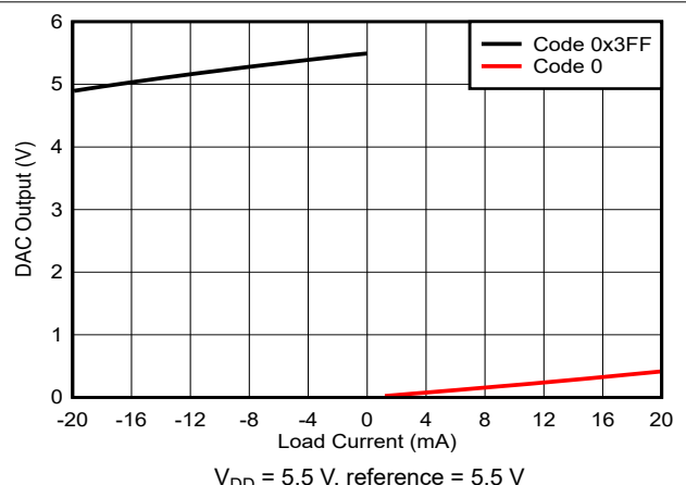
Figure 7-51. Output Source and Sink Capability
