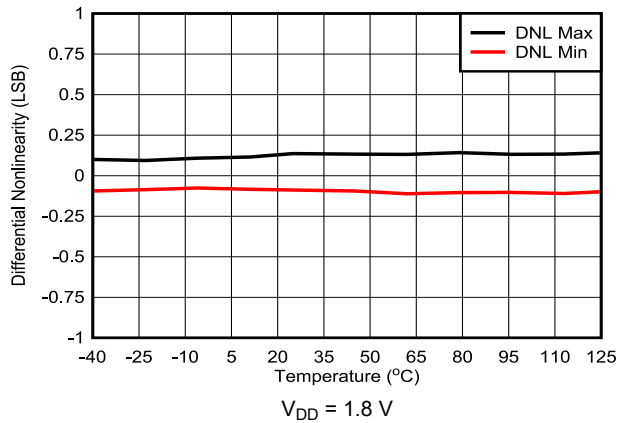
Figure 7-10. Differential Nonlinearity vs Temperature
