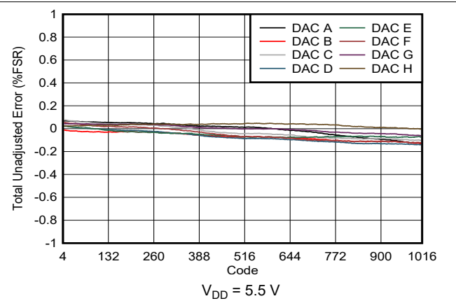
Figure 7-15. Total Unadjusted Error vs Digital Input Code
