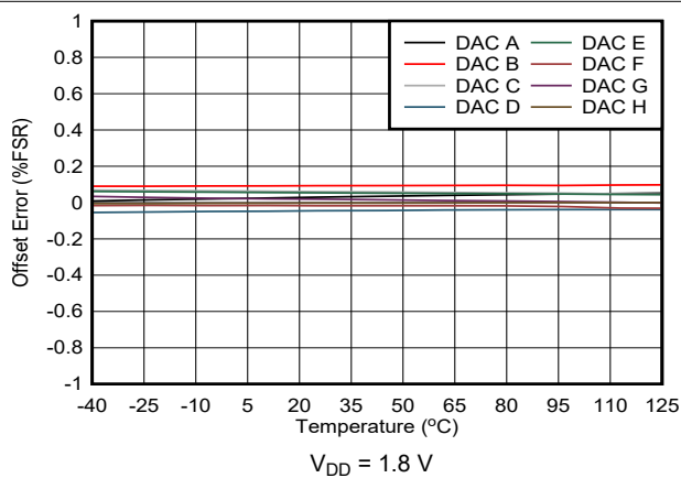
Figure 7-24. Offset Error vs Temperature
