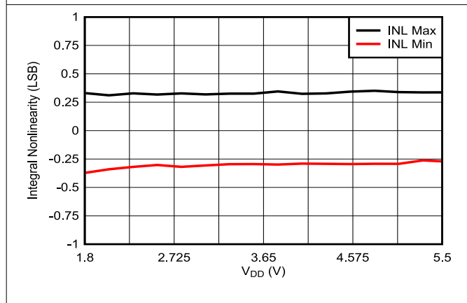
Figure 7-6. Integral Nonlinearity vs Supply Voltage
