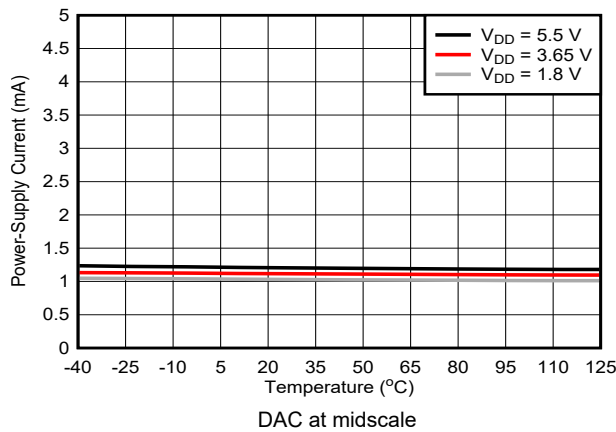
Figure 7-48. Power-Supply Current vs Temperature
