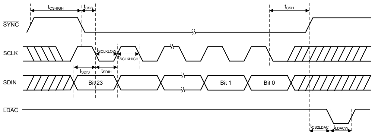
Figure 7-1. Serial Interface Timing Diagram
