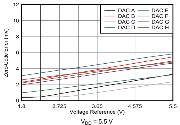
Figure 7-23. Zero-Code Error vs Voltage Reference
