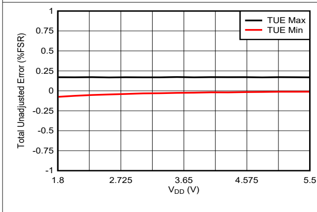
Figure 7-18. Total Unadjusted Error vs Supply Voltage
