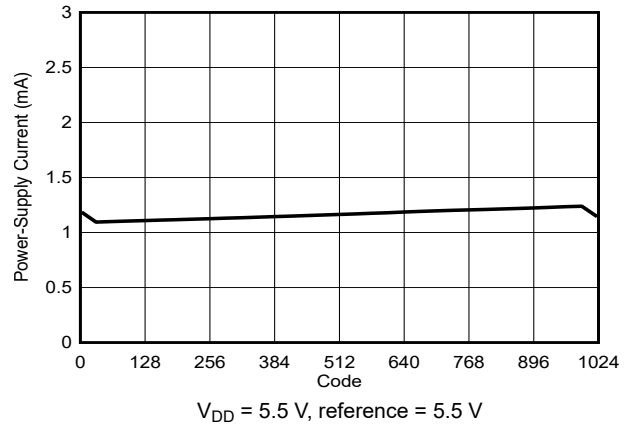
Figure 7-47. Power-Supply Current vs Digital Input Code
