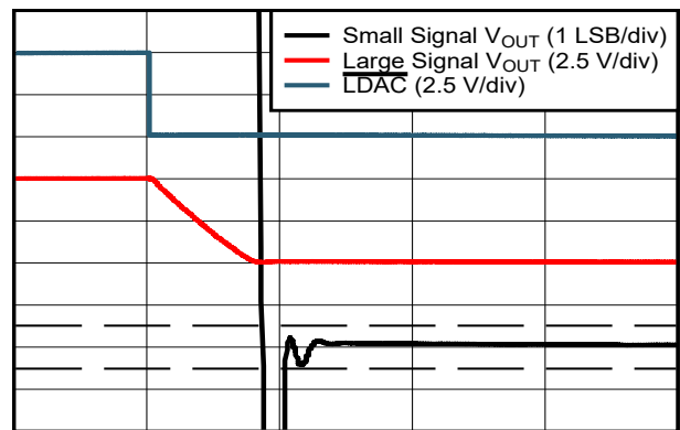
Figure 7-37. Glitch Impulse, Falling Edge, 1 LSB Step
