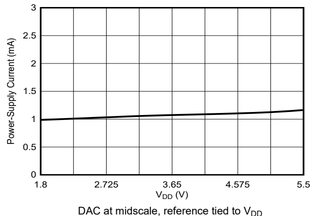
Figure 7-49. Power-Supply Current vs Supply Voltage
