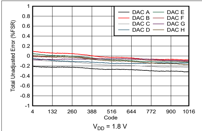
Figure 7-14. Total Unadjusted Error vs Digital Input Code
