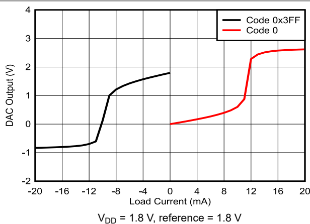
Figure 7-50. Output Source and Sink Capability
