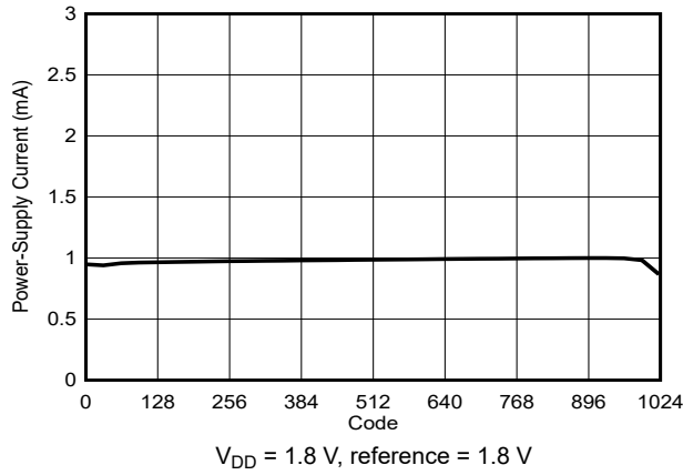
Figure 7-46. Power-Supply Current vs Digital Input Code
