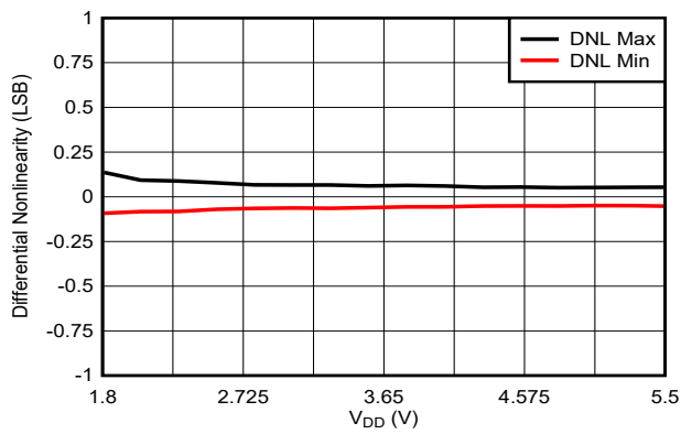
Figure 7-12. Differential Nonlinearity vs Supply Voltage
