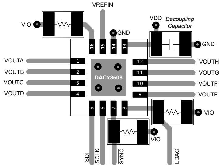
Figure 11-1. Layout Example
