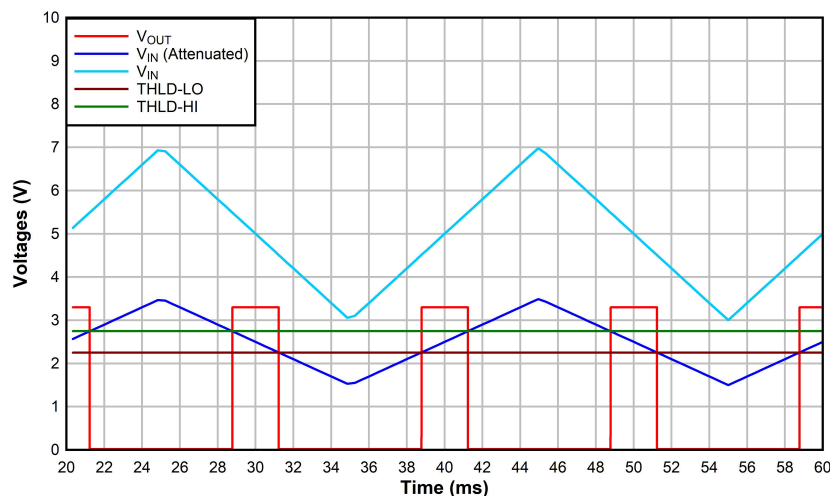
Figure 9-4. Programmable Comparator Output Waveform
