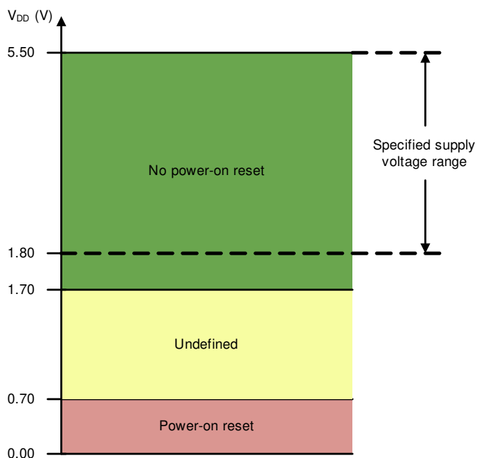
Figure 8-2. Threshold Levels for V_{DD} POR Circuit
