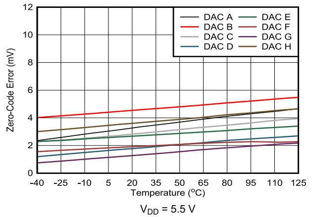
Figure 7-21. Zero-Code Error vs Temperature
