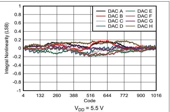
Figure 7-3. Integral Nonlinearity vs Digital Input Code
