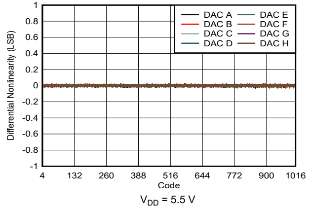
Figure 7-9. Differential Nonlinearity vs Digital Input Code
