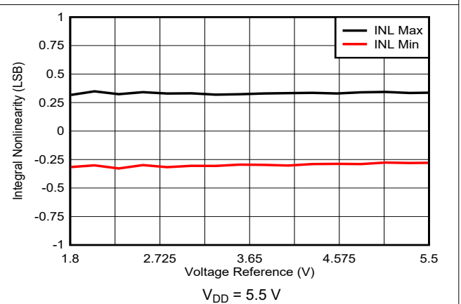
Figure 7-7. Integral Nonlinearity vs Voltage Reference
