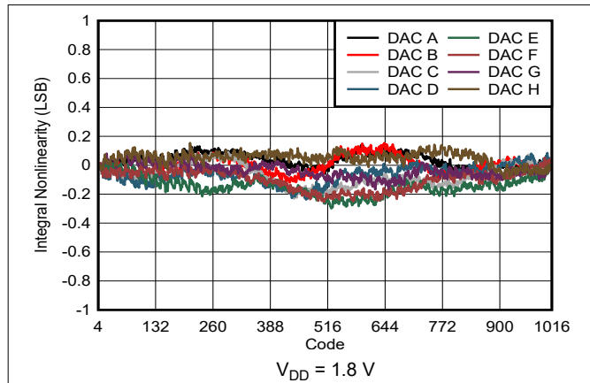
Figure 7-2. Integral Nonlinearity vs Digital Input Code
