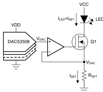
Figure 9-1. Programmable LED Biasing
