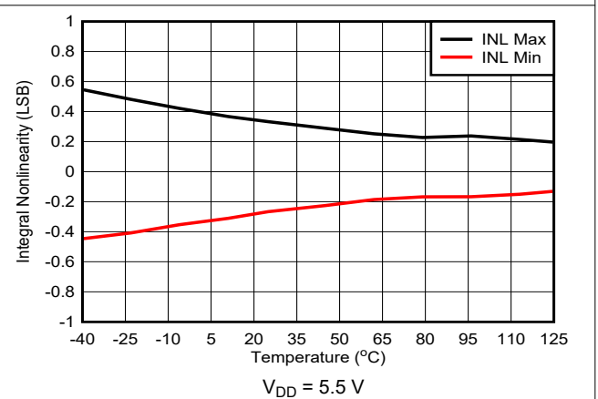
Figure 7-5. Integral Nonlinearity vs Temperature
