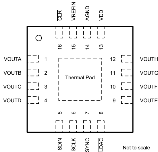
Figure 6-1. RTE (16-Pin WQFN) Package, Top View
