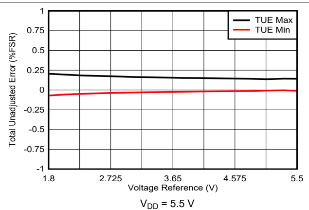
Figure 7-19. Total Unadjusted Error vs Voltage Reference
