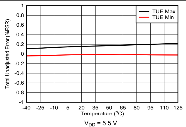
Figure 7-17. Total Unadjusted Error vs Temperature
