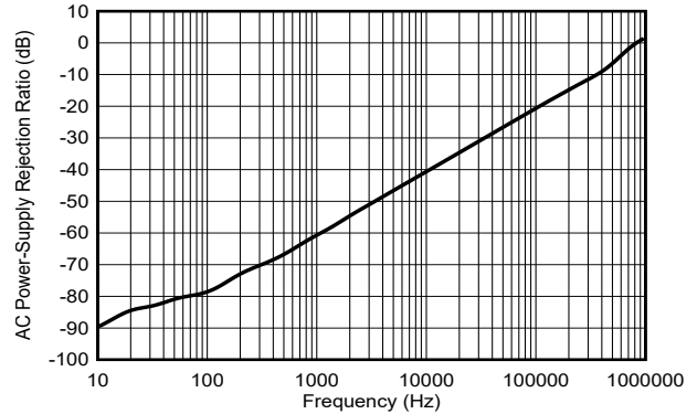
Figure 7-43. AC Power-Supply Rejection Ratio vs Frequency
