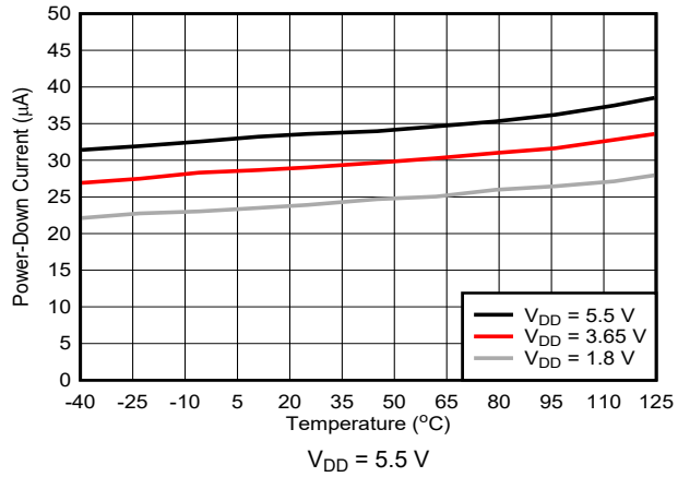
Figure 7-52. Power-Down Current vs Temperature
