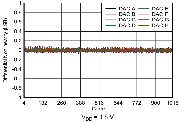
Figure 7-8. Differential Nonlinearity vs Digital Input Code
