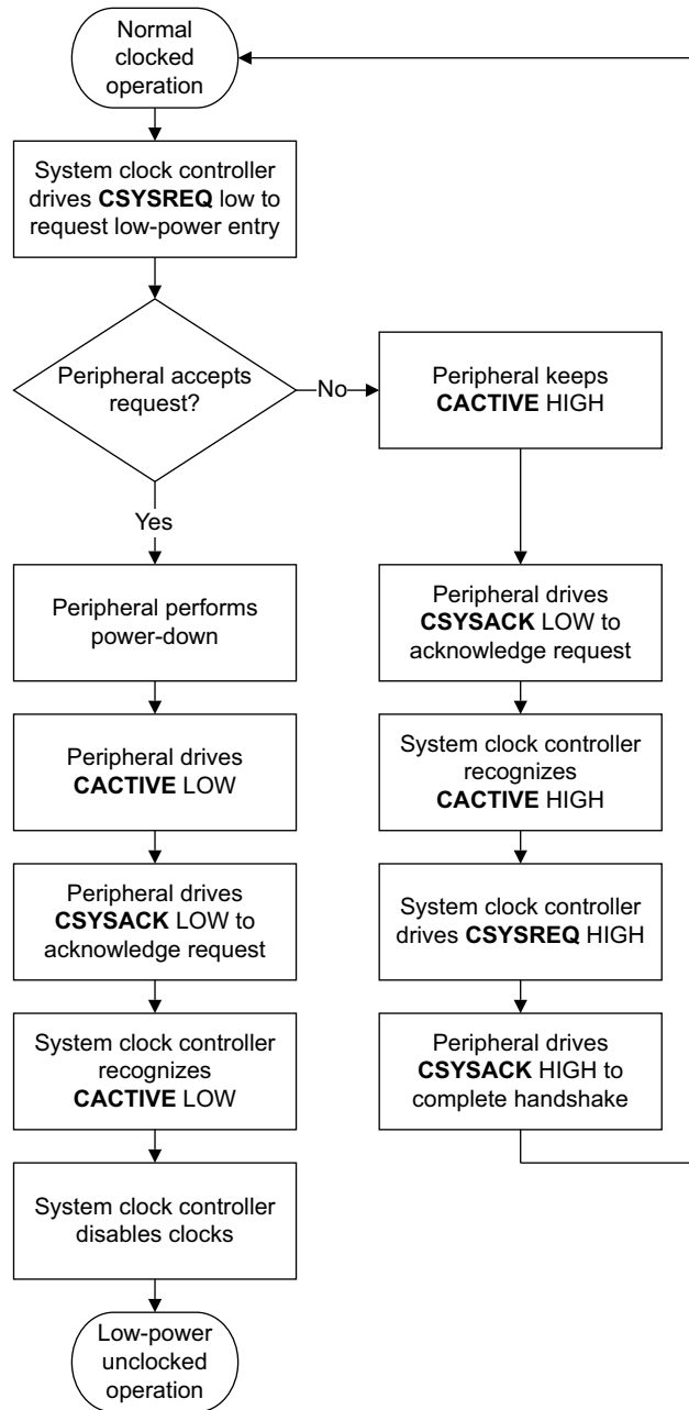
Figure A9-6 Requesting entry to low-power state
