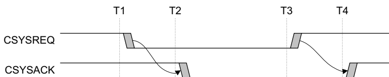
Figure A9-1 CSYSREQ and CSYSACK handshake
